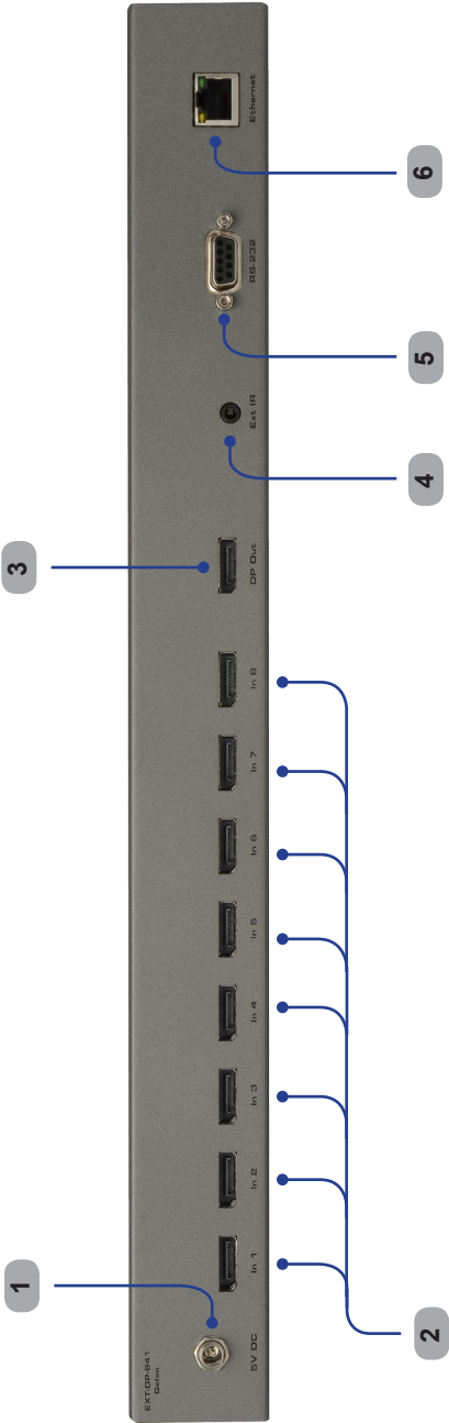
Back Panel
